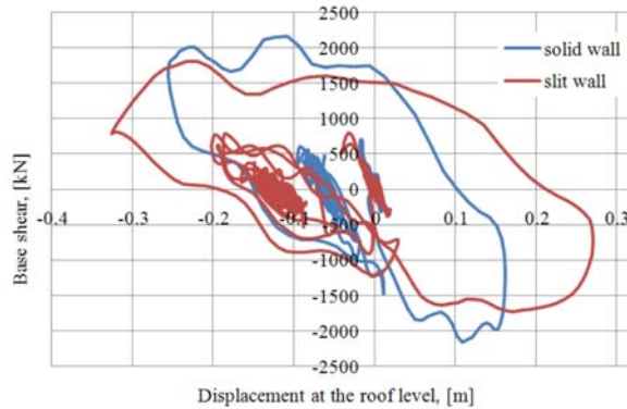
Fig. 13 – Hysteretic behaviour of the walls at Vrancea 1977 N-S earthquake, PGA = 0.3 g.
